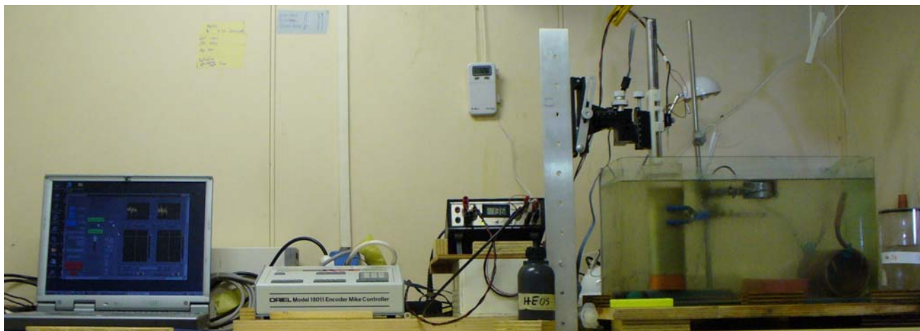
Fig. 6-1. Set-up of the experimental system for measuring oxygen microprofiles in a sediment core. It includes a picoammeter (PA2000) to read the signal, a heavy/stable laboratory stand and a motorized micromanipulator. The analogic signal from the picoammeter is converted to digital from the A/D converter and acquired from specific software. The software controls also the motorized micromanipulator and the penetration of the micro sensor into the sediment. The sediment core is positioned within a thermostated bath kept at the temperature of the sea bottom.
