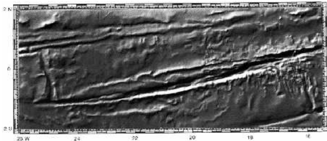
Figure 4. Shaded relief map of the Romanche Transform Region, derived by bathymetric data. Shaded relief map was obtained assuming illumination from NW 45° over the horizon. Horizontal resolution is 1KM, no vertical exaggeration. Mercator projection at 0°.
